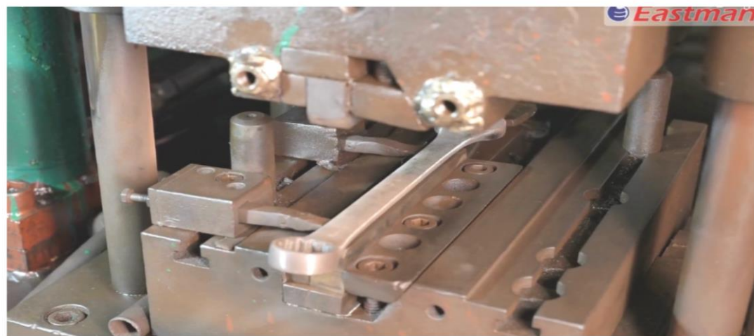
COLD STAMPING – BRANDING 200 + 400 ton Hydraulic press for brand Embossing by cold forging.
